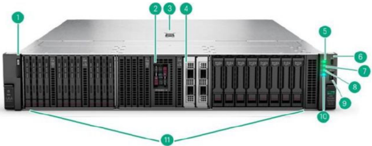
Front View - SFF/EDSFF CTO Server
